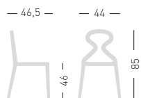
ANITA Techno polymer chair. Sedia integrale in tecnopolimero.
