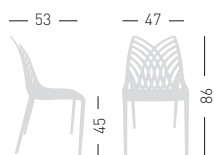
OPERA 4-Legged techno polymer chair. Sedia 4 gambe in tecnopolimero.
